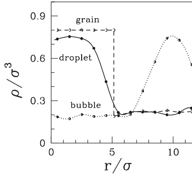
FIG. 5. The profile of the total density corresponding to (a) a droplet of liquid A immersed in fluid B (the solid line), (b) a bubble of fluid B immersed in liquid A (the dotted line), and (c) a spherical solid, of the same number of particles as the droplet, immersed in fluid B (the dashed line). The molecules occupy the pore space and the axial average has been performed—the profile is plotted vs the radius. The droplet data show an enhancement in the density next to the wall that corresponds to the first monolayer peak indicated in Fig. 2 without the axial averaging.
