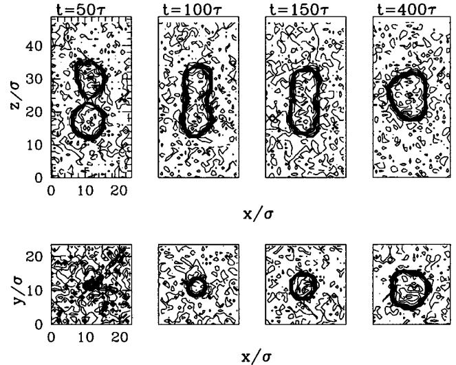
FIG. 6. The density contours of the droplets during coalescence. The data were time averaged over periods of 25\tau . The top panels refer to a central cut in the xz plane. The bottom panels refer to a plane that is halfway between the initially separated droplets and later becomes an equatorial plane in the fused droplet.
