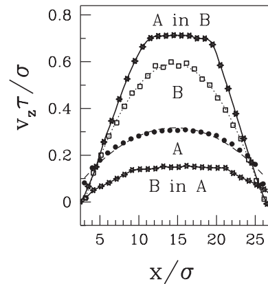
FIG. 12. The velocity profiles when g of 0.01\epsilon/\sigma is applied to all atoms within the pore. The top and bottom curves refer to the droplet and bubble cases, respectively. The data points marked by A and B are the same as in the lower panel of Fig. 2.
