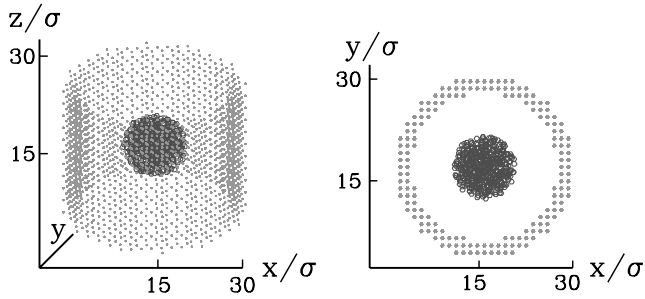
FIG. 1. A snapshot of solid sphere moving through a fluid-filled cylindrical pore. Only the solid and wall atoms are shown for clarity. The solid consists of 454 atoms that are tethered to amorphously placed centers. There are 2212 pore wall atoms which are fixed rigidly. The space between the solid and the pore is filled with 2281 fluid atoms (the case of fluid B). The left-hand figure represents a stereographic projection whereas the right-hand figure represents a projection from the top.
