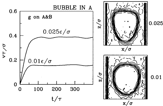
FIG. 11. Same as in Fig. 9 but for g applied to all atoms within the pore space.
